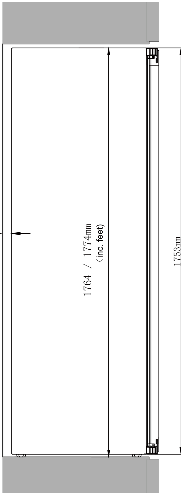
Side View
