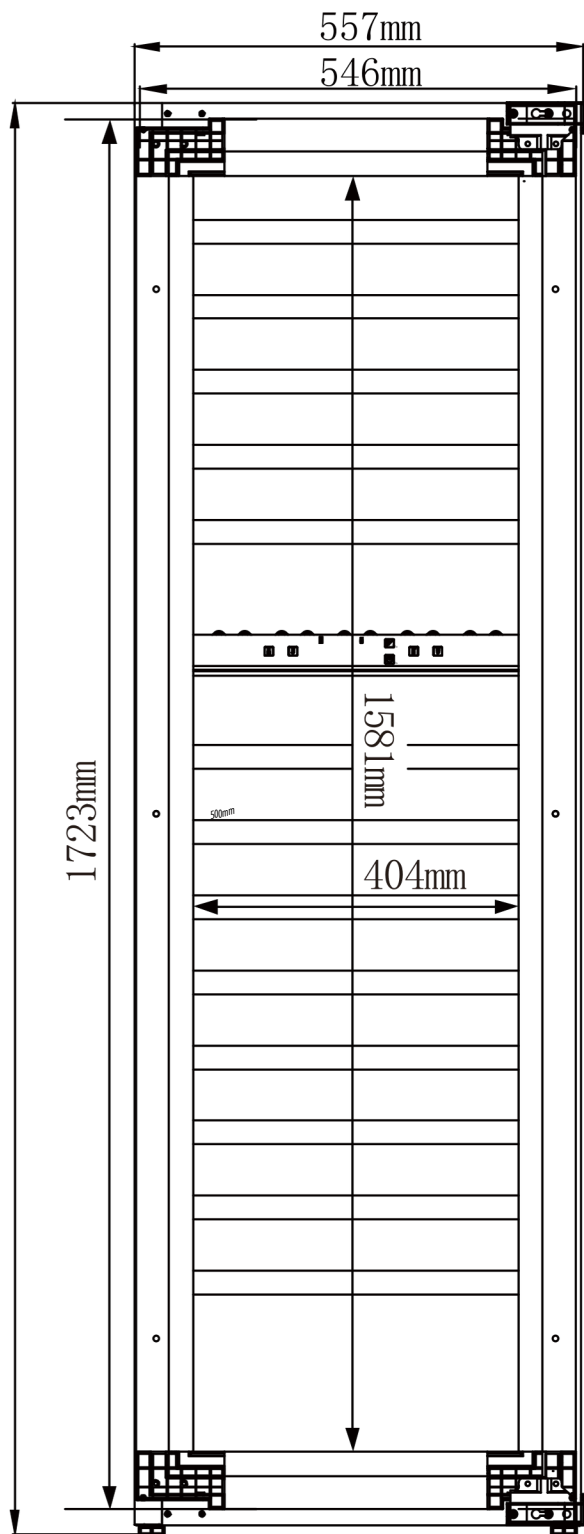
Front View
